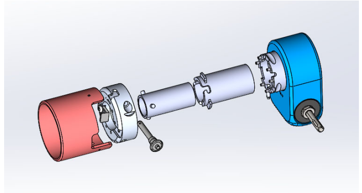
Exploded Component View
